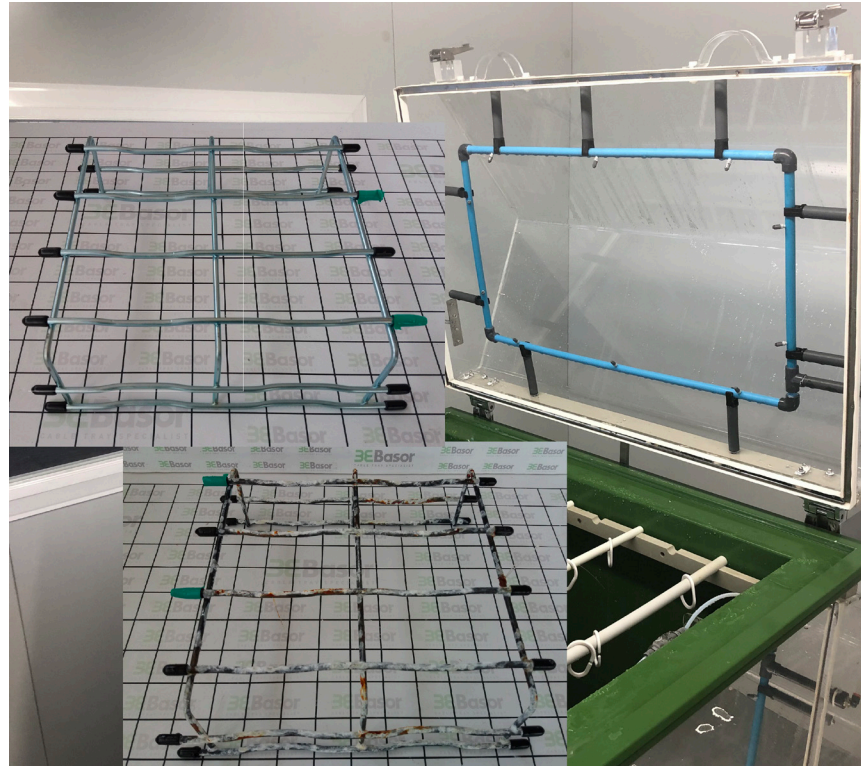
Accelerated corrosion test in a salt spray chamber.
