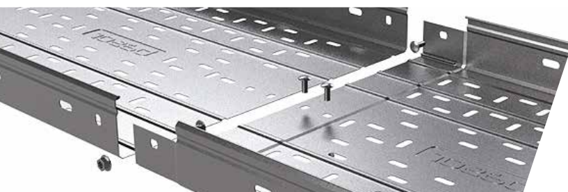
Impedance at the junction between pieces less than 50 mΩ
