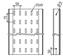
B 200/300
