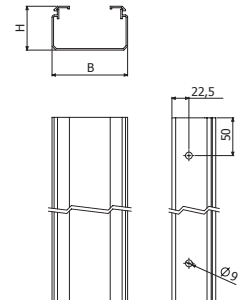
B 100/150
